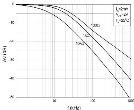
Fig.11 Frequency Response
